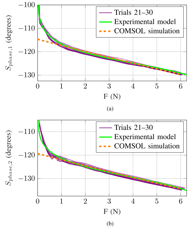
Fig. 8. Plots of the experimental results for trials 21 to 30, model created from the experimental data, and the results of the FEA for (a) sensor 1 and (b) sensor 2.
